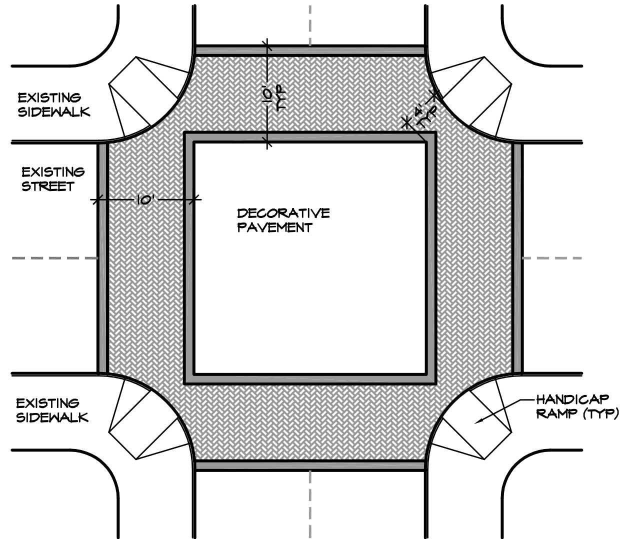
TYPICAL CROSSWALK - PLAN VIEW SCALE: 1 IN = 10 FT
